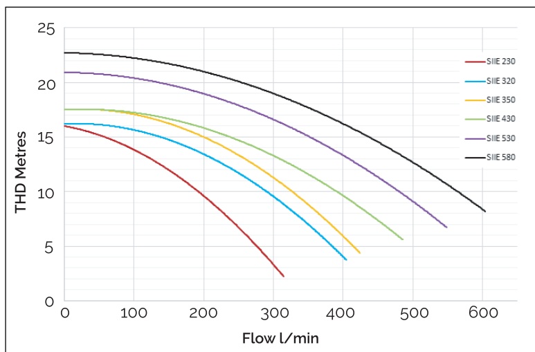
Flow Charts
